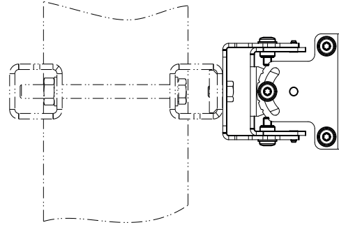
b) Pole Mounting with Optional Mast Clamp (Order No. 52010368)
